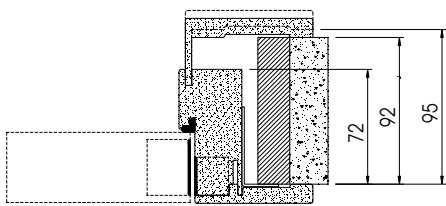
Tavolato 72 Sp. parete min. 92 max. 95 Board 72, wall thickness min. 92 max. 95
