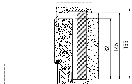
Tavolato 132 Sp. parete min. 132 max. 155 Board 132, wall thickness min. 132 max. 155
