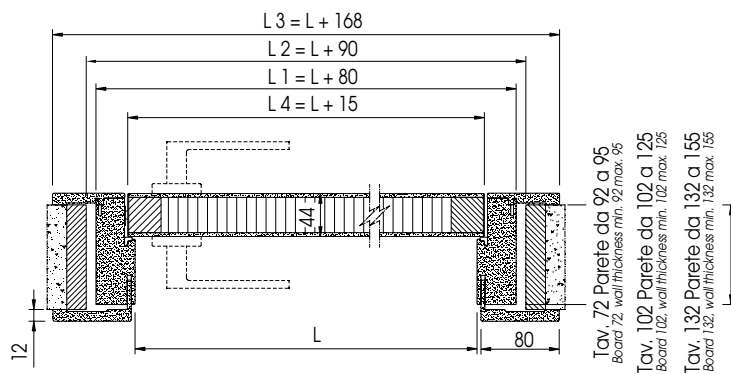
Tavolato 72 Sp. parete min. 92 max. 95 Board 72, wall thickness min. 92 max. 95
